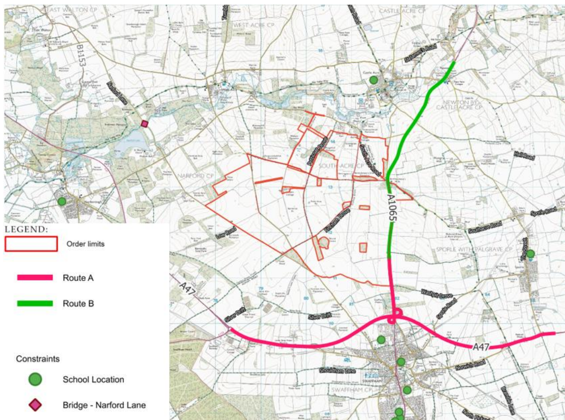
Figure 4-1 Proposed Construction Routing Overview
